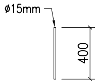
PIN DETAIL
