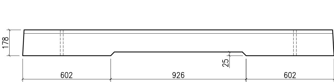
SIDE VIEW A
