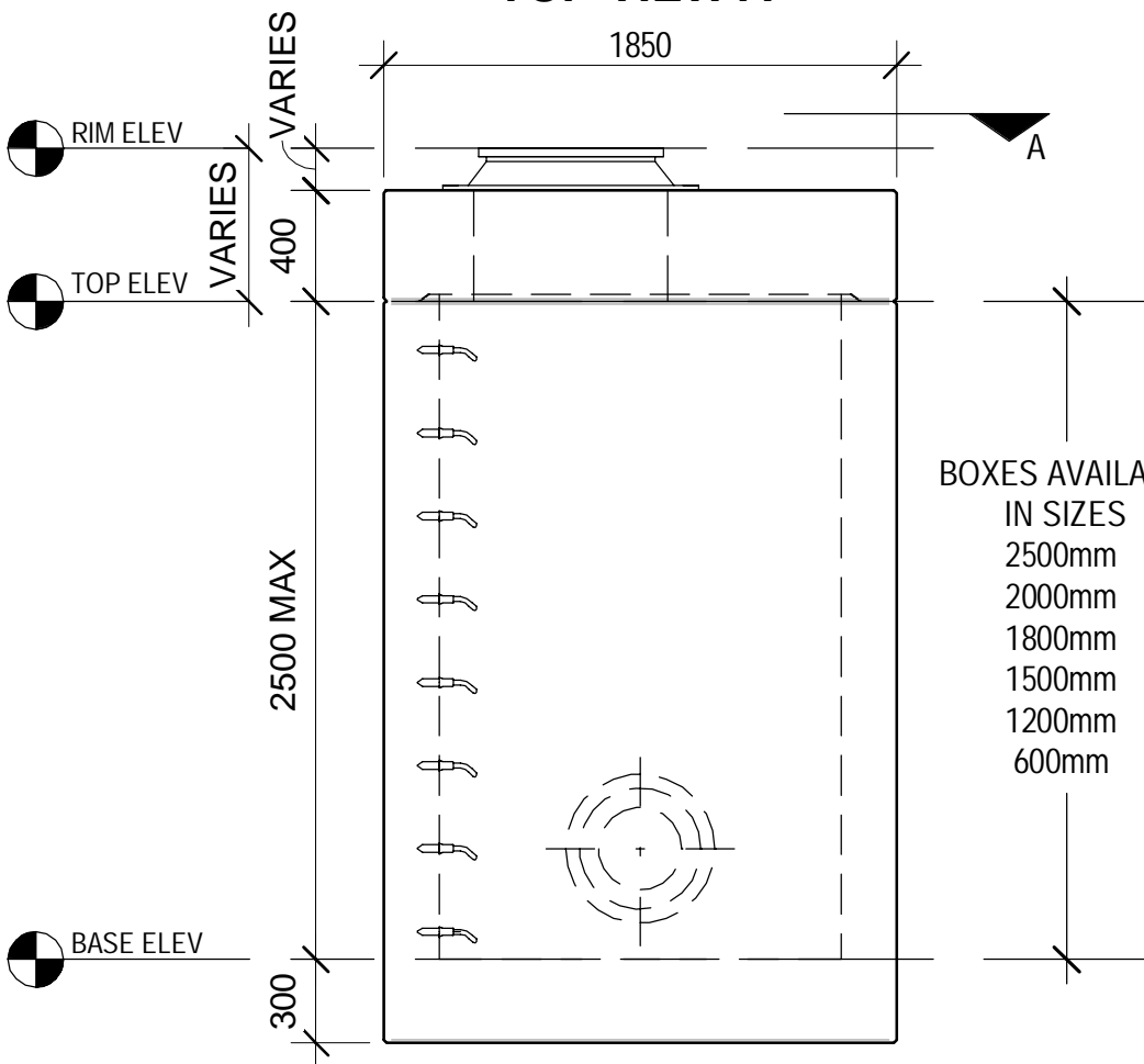
FRONT ELEVATION
