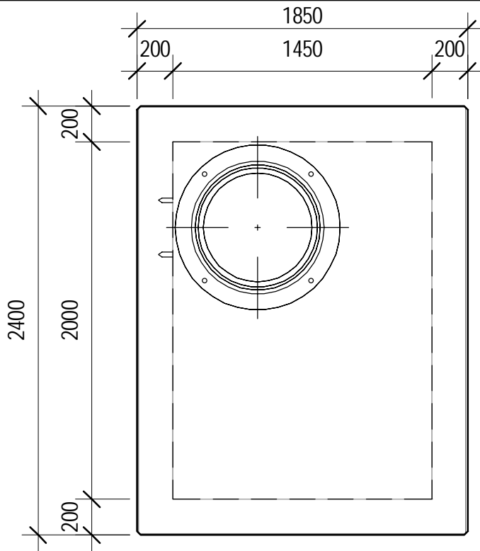
TOP VIEW A
