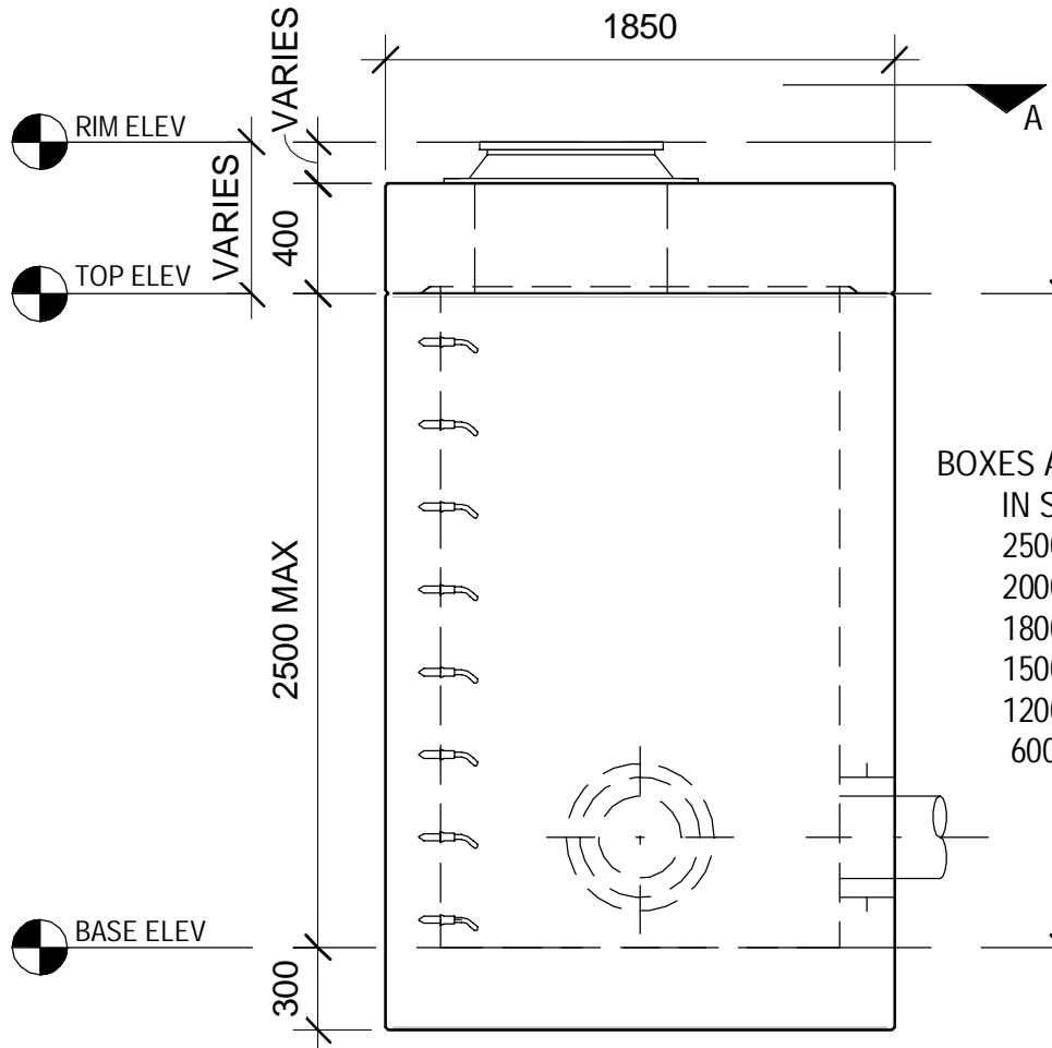
FRONT ELEVATION
